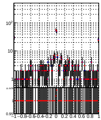
DQM_TT_mkFit_ DQM_TT_mkFit_BDT_
