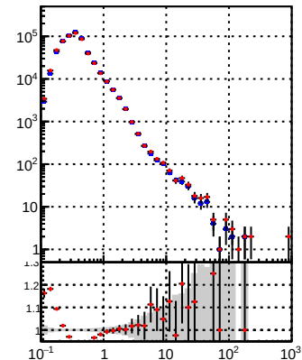
—●— DQM_TT_mkFit —●— DQM_TT_mkFit BDT
