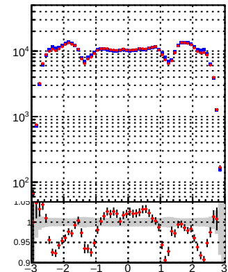
—●— DQM_TT_mkFit —●— DQM_TT_mkFit BDT
