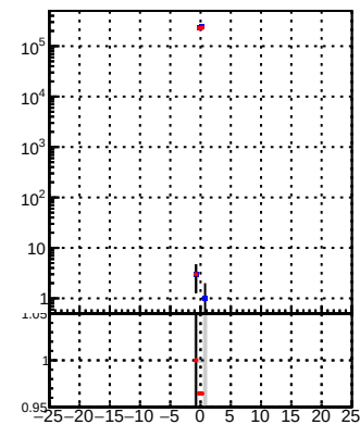
DQM_TT_mkFit_ DQM_TT_mkFit_BDT_
