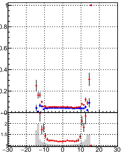
Fake rate vs \sqrt{s} —●— DQM_TT_mkFit —●— DQM_TT_mkFit_BDT
