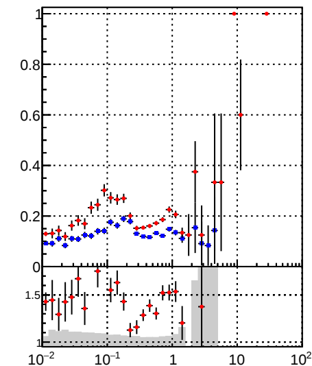
—•— DQM_TT_mkFit_ —•— DQM_TT_mkFit_BDT_
