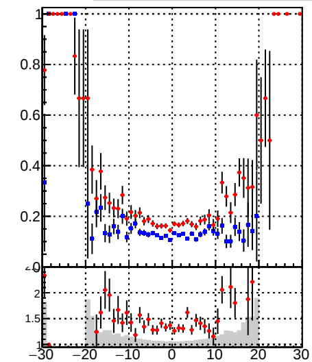
—•— DQM_TT_mkFit_ —•— DQM_TT_mkFit_BDT_
