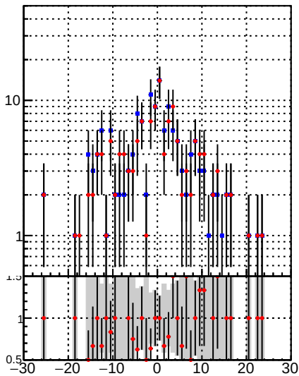
N of associated tracks (simToReco) vs z vert position
