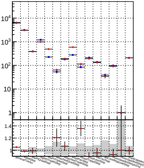
Number —●— DQM_TT__mkFit_BDT
