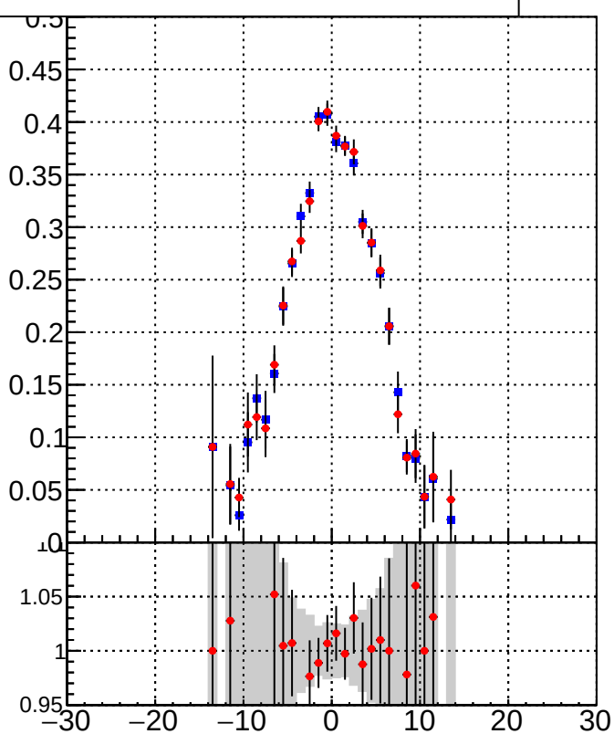
fake+duplicates vs dz
