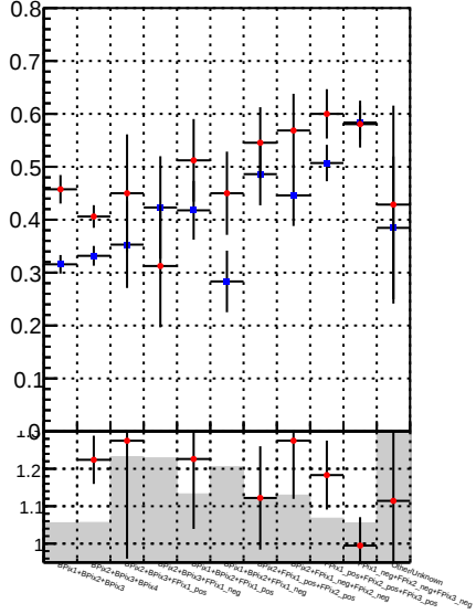
Fake rate vs. DQM_TT_mkFit DQM_TT_mkFit_BDT
