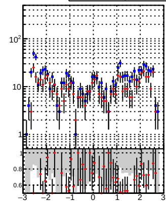
N of reco track vs \eta Legend: DQM TT mkFit (blue) DQM TT mkFit BDT (red)
