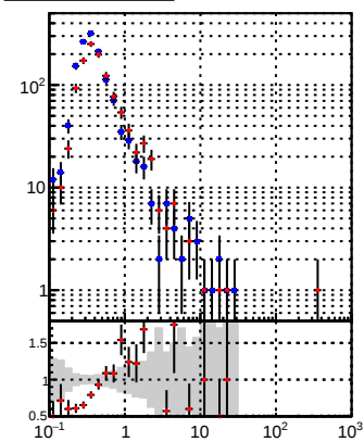
—•— DQM_TT_mkFit —•— DQM_TT_mkFit_BDT
