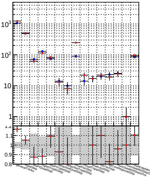
Number —●— DQM_TT__mkFit_BDT_
