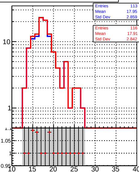
N of reco track vs pT
