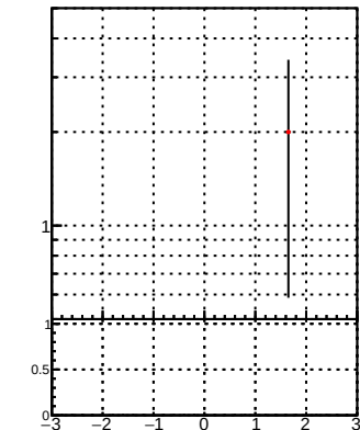
N of associated (recoToSim) duplicate tracks vs \eta ps eta
