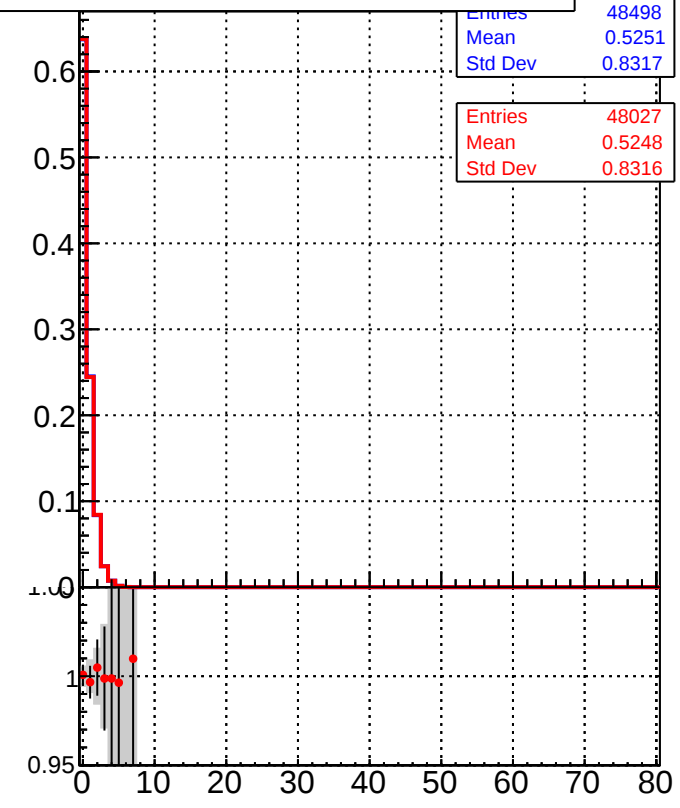
DQM_TT_mkFit_ DQM_TT_mkFit_BDT_
