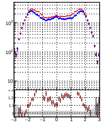
N of reco track vs \eta —•— DQM_TT_mkFit —•— DQM_TT_mkFit_BDT
