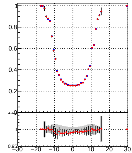
■ DQM_TT_mkFit_ ● DQM_TT_mkFit_BDT_ Fake rate vs vertpos
