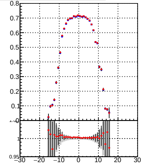
■ DQM_TT_mkFit_ ● DQM_TT_mkFit_BDT_ Pileup rate vs vertpos
