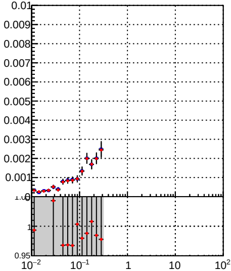
■ DQM_TT_mkFit_ ● DQM_TT_mkFit_BDT_ Duplicates Rate vs vertpos
