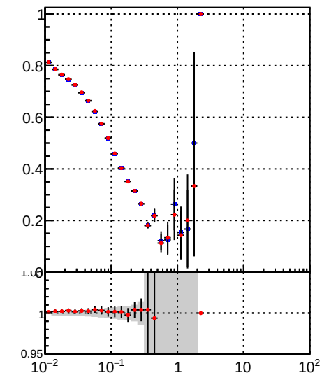
■ DQM_TT_mkFit_ ● DQM_TT_mkFit_BDT_ Pileup rate vs vertpos
