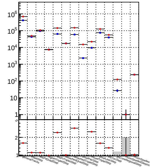
Number —●— DQM_TT__mkFit_BDT_
