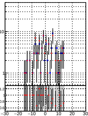
N of associated (recoToSim) loop tracks vs dz
