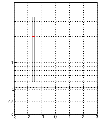
N of associated (recoToSim) duplicate tracks vs \eta ◆ DQM TT mkFit × DQM TT mkFit BDT
