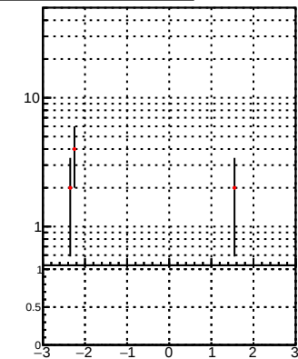
—•— DQM_TT_mkFit —•— DQM_TT_mkFit_BDT
