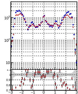
N of reco track vs \eta Legend: DQM_TT_mkFit (blue diamonds) DQM_TT_mkFit_BDT (red crosses)
