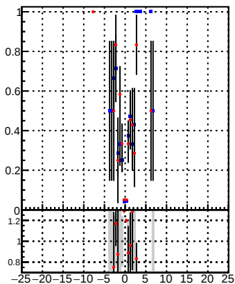
—●— DQM_TT_mkFit_ —●— DQM_TT_mkFit_BDT_
