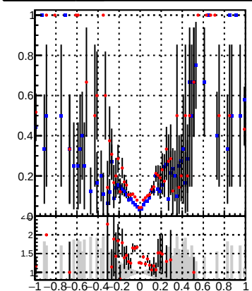
—●— DQM_TT_mkFit_ —●— DQM_TT_mkFit_BDT_
