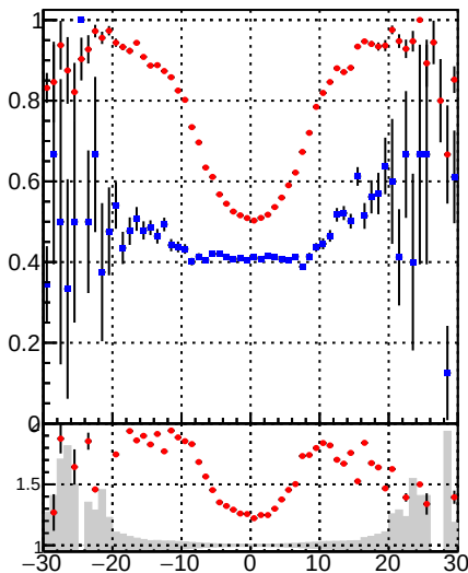
—•— DQM_TT_mkFit_ —•— DQM_TT_mkFit_BDT_
