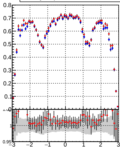
— DQM_DisplacedSUSY__mkFit_BDT_ — DQM_DisplacedSUSY__mkFit_
