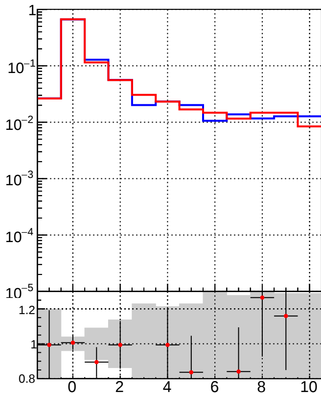
TruePVLocationIndexInRecoVertexCollection
