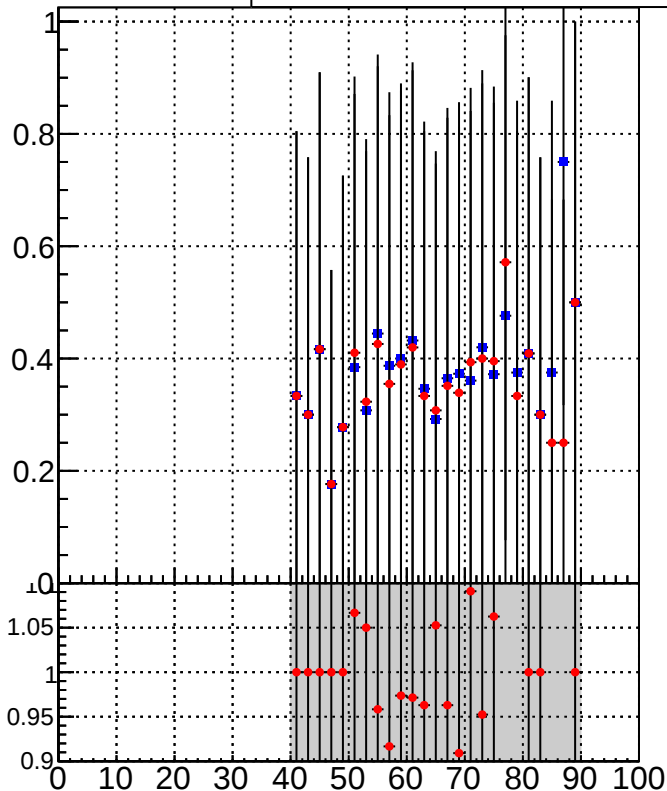
—■— DQM_DisplacedSUSY_mkFit_BDT_ —●— DQM_DisplacedSUSY_mkFit_
