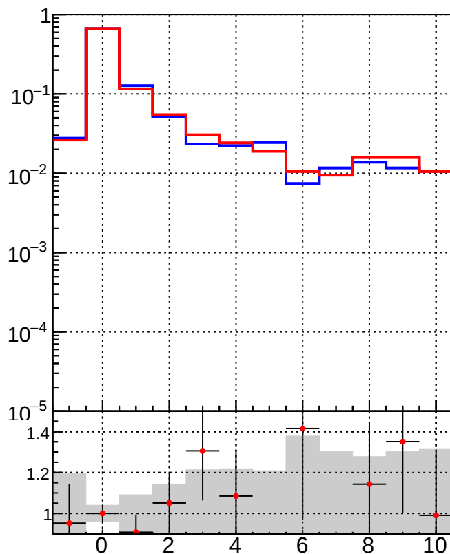
TruePVLocationIndexInRecoVertexCollection
