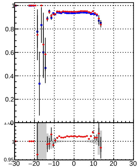
—■— DQM_DisplacedSUSY_mkFit_BDT_ —●— DQM_DisplacedSUSY_mkFit_
