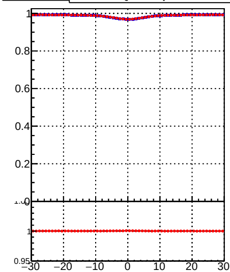
—•— DQM_DisplacedSUSY_mkFit_BDT_
