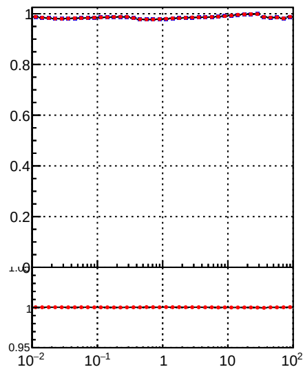
—•— DQM_DisplacedSUSY_mkFit_BDT_
