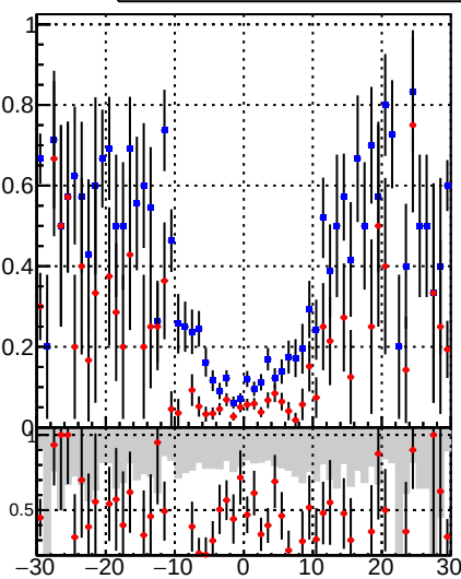
—■— DQM_DisplacedSUSY_mkFit_BDT_ —●— DQM_DisplacedSUSY_mkFit_
