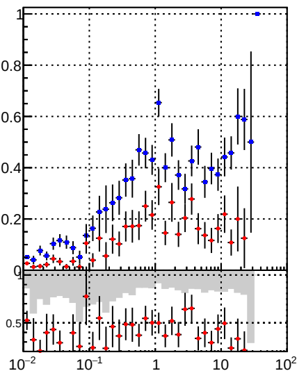
—■— DQM_DisplacedSUSY_mkFit_BDT_ —●— DQM_DisplacedSUSY_mkFit_
