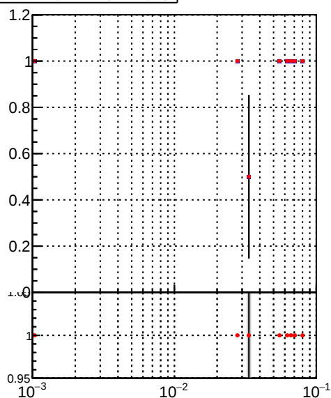
Efficiency vs d_r(\text{track, jet})
