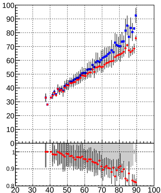
RecoVtx_vs_GenVtx
