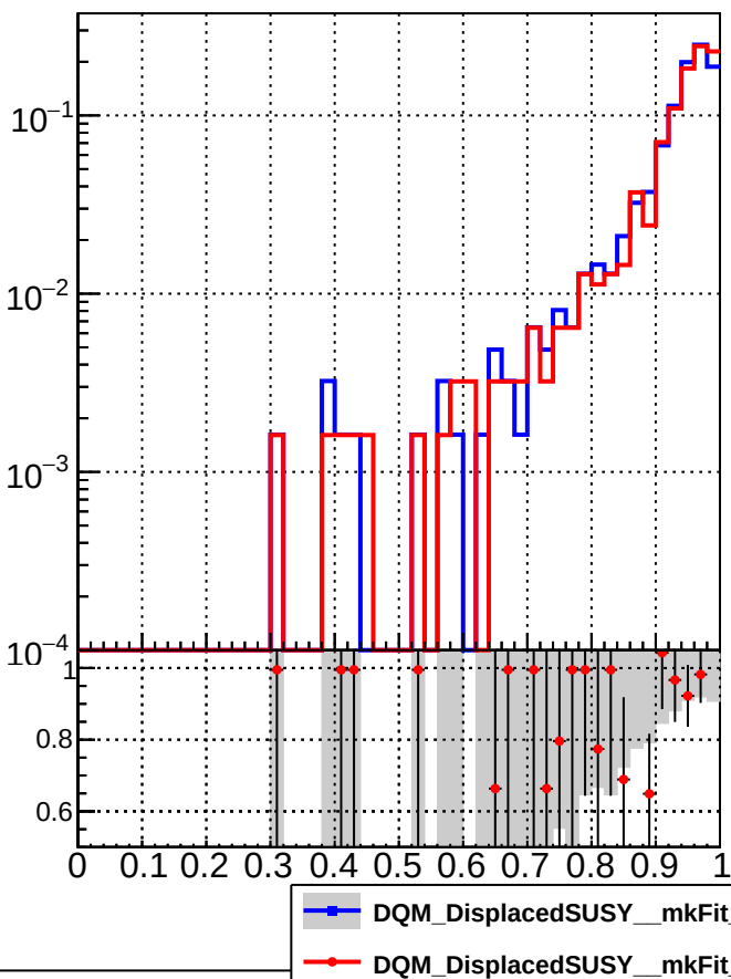
RecoPVAssoc2GenPVMatched_Missing
