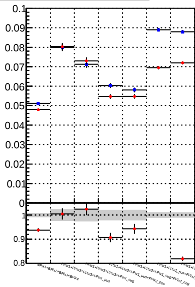
Fake rate vs. —•— DQM_DisplacedSUSY_mkFit_BDT_ —•— DQM_DisplacedSUSY_mkFit_
