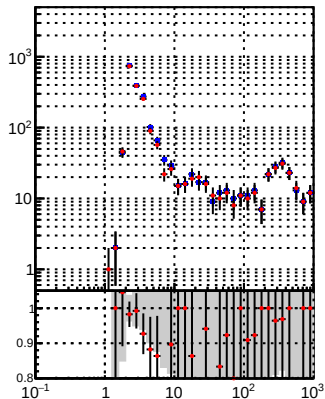
—●— DQM_DisplacedSUSY_mkFit_BDT_ —●— DQM_DisplacedSUSY_mkFit
