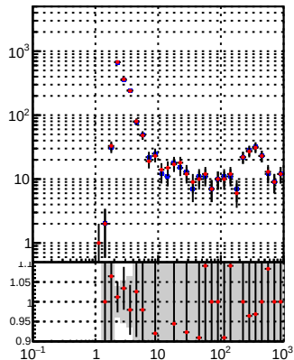
—●— DQM_DisplacedSUSY_mkFit_BDT_ —●— DQM_DisplacedSUSY_mkFit
