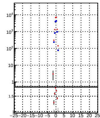
—•— DQM_DisplacedSUSY_mkFit_BDT_
