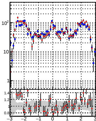
N of reco track vs \eta pT [GeV] —●— DQM_DisplacedSUSY_mkFit_BDT_ —+— DQM_DisplacedSUSY_mkFit
