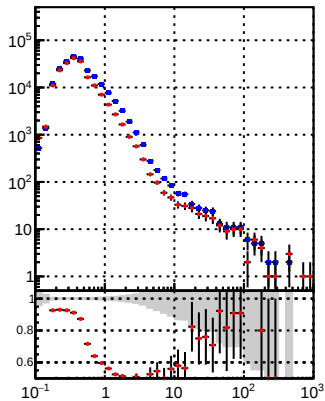
N of reco track vs \eta pT [GeV] —•— DQM_DisplacedSUSY_mkFit_BDT_ —•— DQM_DisplacedSUSY_mkFit
