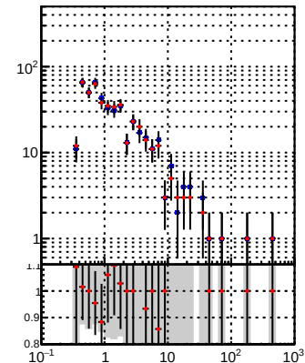
—●— DQM_DisplacedSUSY_mkFit_BDT_ —●— DQM_DisplacedSUSY_mkFit
