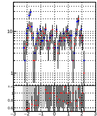
N of reco track vs \eta —●— DQM_DisplacedSUSY_mkFit_BDT_ —●— DQM_DisplacedSUSY_mkFit
