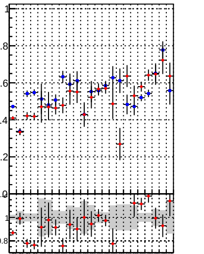
Fake rate vs. DQM_DisplacedSUSY_mkFit_BDT_ DQM_DisplacedSUSY_mkFit_
