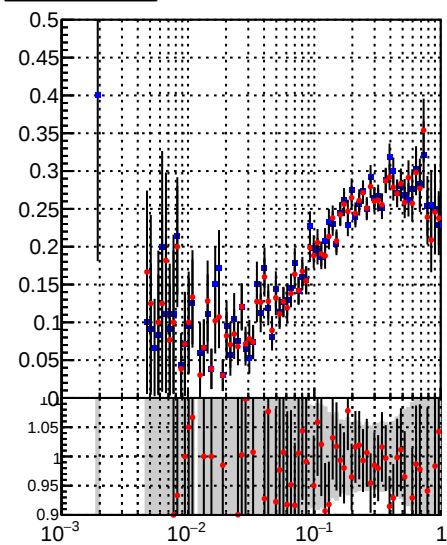
Fake rate vs \sqrt{s} Legend: DQM_DisplacedSUSY_mkFit_BDT_ (blue squares) DQM_DisplacedSUSY_mkFit_ (red circles)
