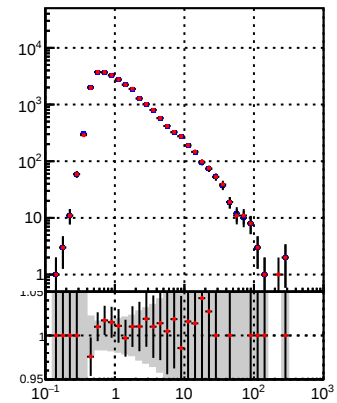
N of reco track vs \eta pT eta —•— DQM_DisplacedSUSY_mkFit_BDT_ —•— DQM_DisplacedSUSY_mkFit
