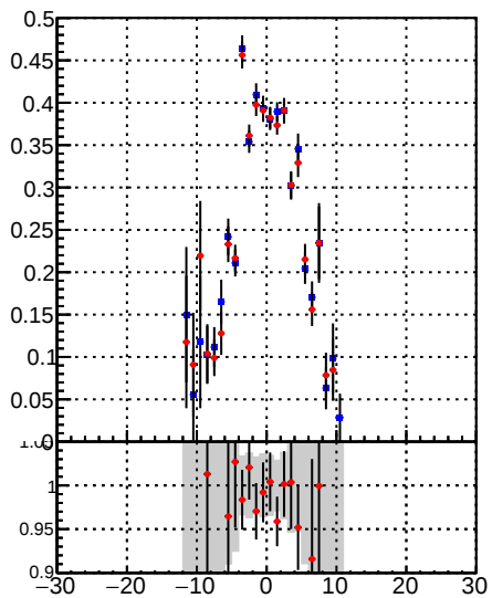
Fake rate vs d —●— DQM_DisplacedSUSY_mkFit_BDT_ —●— DQM_DisplacedSUSY_mkFit_
