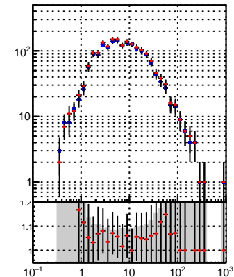
—●— DQM_DisplacedSUSY_mkFit_BDT_
