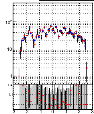
—●— DQM_DisplacedSUSY_mkFit_BDT_
