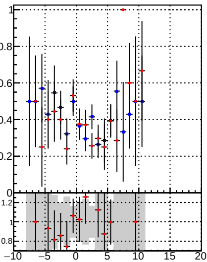
Fake rate vs. sim PV z
