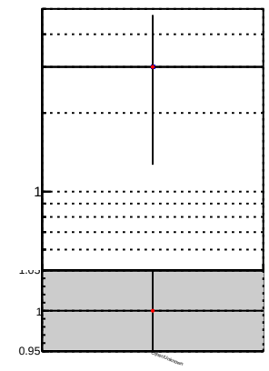
N of reco track vs. \chi^2 for DQM DisplacedSUSY mkFit BDT and DQM DisplacedSUSY mkFit
