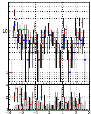
N of reco track vs \eta DQM_DisplacedSUSY_mkFit_BDT_ DQM_DisplacedSUSY_mkFit
