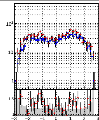
N of reco track vs \eta DQM_DisplacedSUSY_mkFit BDT DQM_DisplacedSUSY_mkFit pT eta
