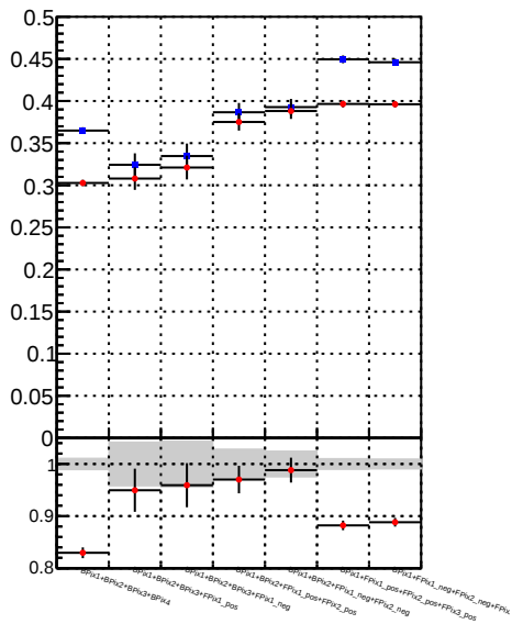
Fake rate vs. —♦— DQM_DisplacedSUSY_mkFit_BDT_ —x— DQM_DisplacedSUSY_mkFit_
